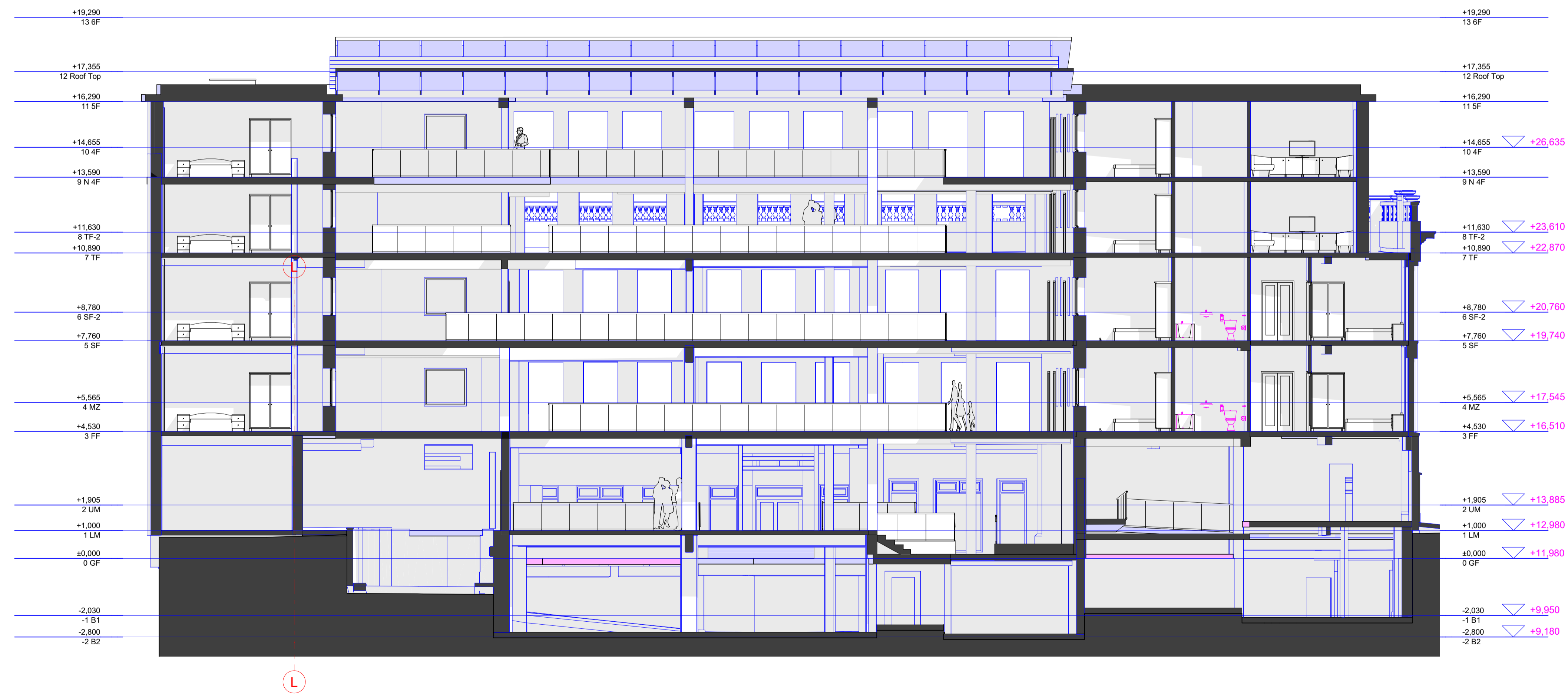
Building Section
