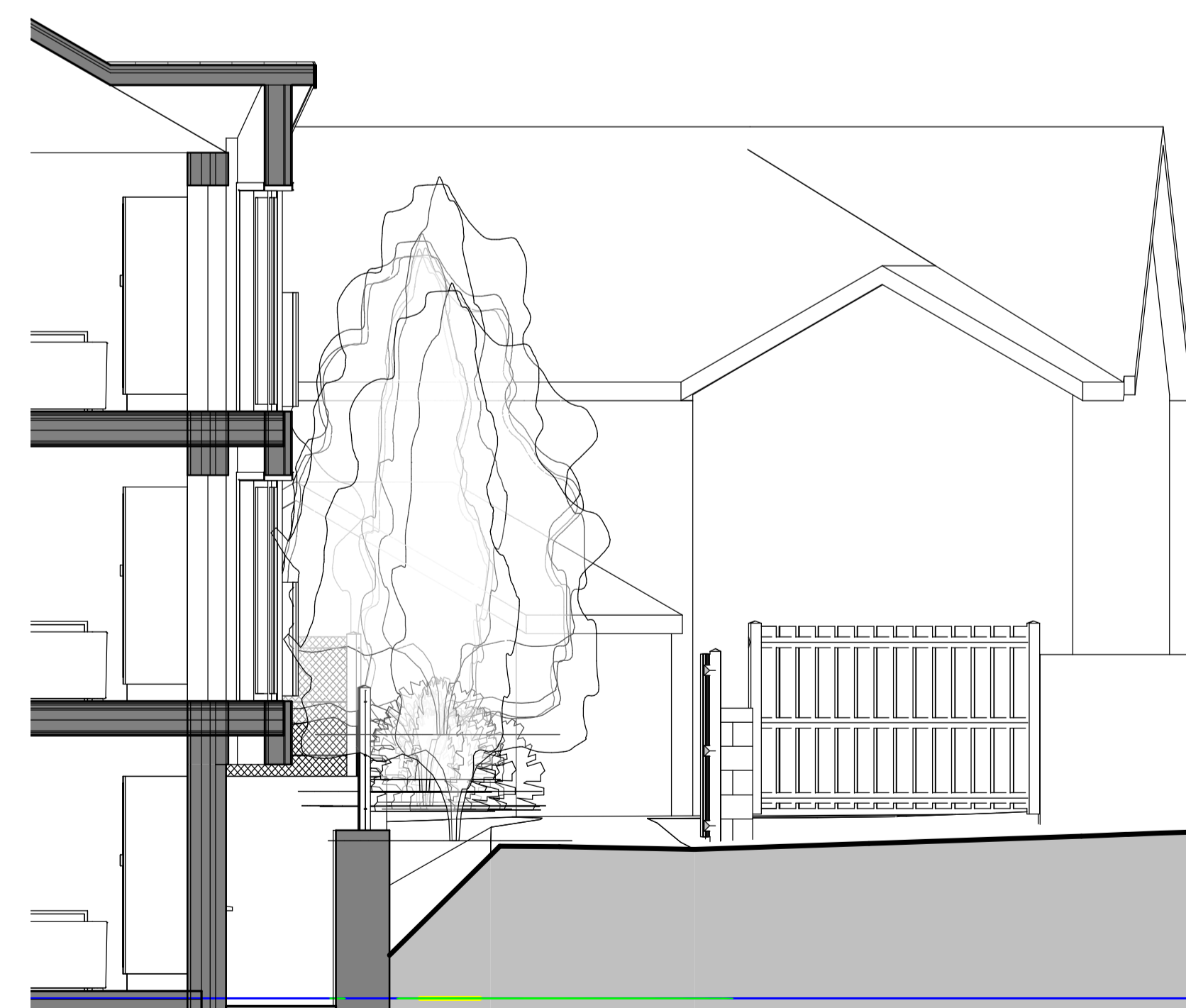
B Section B - Block 4 Lounge 1:50
