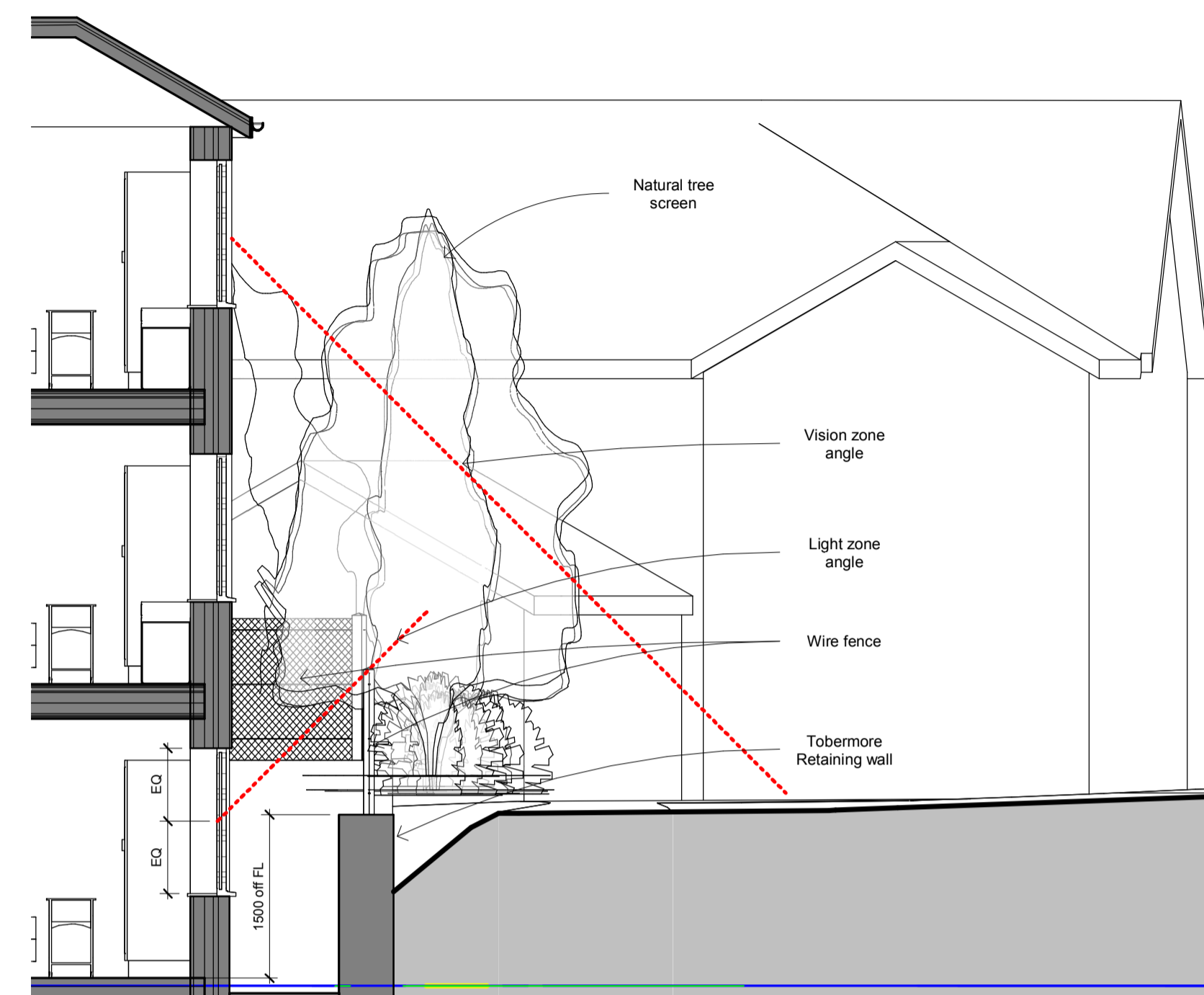
A Section A - Block 4 Bedroom 1:50
